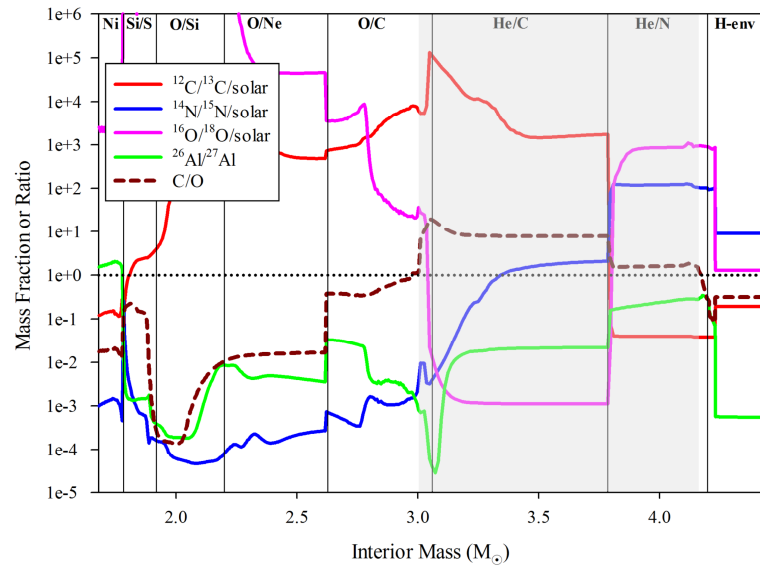
Fig. 1. Theoretical profiles of 26 Al/ 27 Al ratio and solar-normalized C, N, O isotopic composition in the interior of a 15 M_{\odot} pre-explosion SN model [29]. The layer names are indicated along the top of the plot. The shaded region indicates layers where C > O. Mixing between the He/C and He/N zones cannot reproduce the isotopic compositions of some graphite grains as described in the text.
