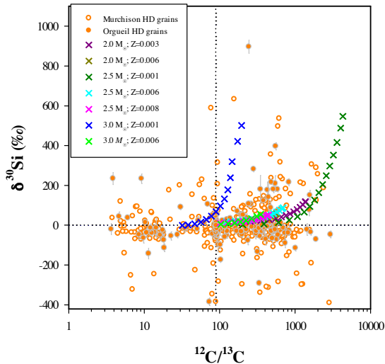
Fig. 2. C and Si isotopic compositions of HD graphite grains compared with F.R.U.I.T.Y. AGB models [43]. ^{12}\text{C} and ^{30}\text{Si} excesses indicate an origin in low-metallicity AGB stars. Dashed lines indicate solar values.
