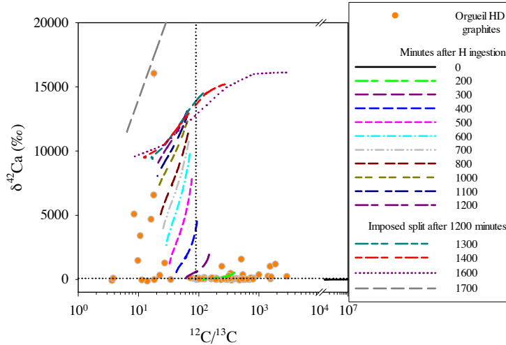
Fig. 3. Ca and C isotopic ratios measured in HD presolar graphite grains compared to VLTP nucleosynthesis model predictions [58]. Each line represents an isotopic depth profile calculated by the VLTP models of the He intershell at a given time (in minutes) after the start of H-ingestion. Grains with extreme Ca anomalies are ^{13}\text{C} -enriched while those with moderate anomalies are mostly ^{12}\text{C} -enriched. Dashed lines indicate solar values.
