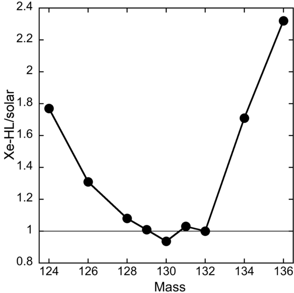
Figure 1. Xe-HL (Huss & Lewis, 1994a). Xenon isotopes are normalized by ^{132}\text{Xe} and by the solar ratios. Xe-HL shows pronounced excesses in the light isotopes ^{124}\text{Xe} and ^{126}\text{Xe} , and in the heavy isotopes ^{134}\text{Xe} and ^{136}\text{Xe} . The excess in ^{124}\text{Xe} and ^{126}\text{Xe} is often referred as Xe-L, that in ^{134}\text{Xe} and ^{136}\text{Xe} as Xe-H.
