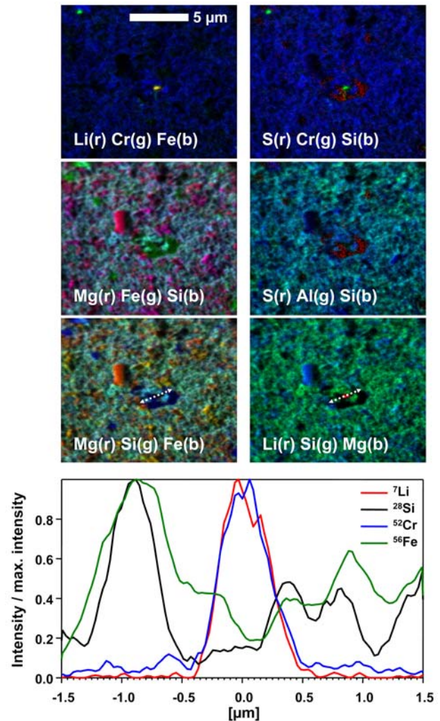
Fig. 5. ToF-SIMS profile across the Li-enriched grain. The position of the one-dimensional profile is indicated in the bottom set of three-color maps. The secondary ion intensities have been normalized within the given range of the profile.
