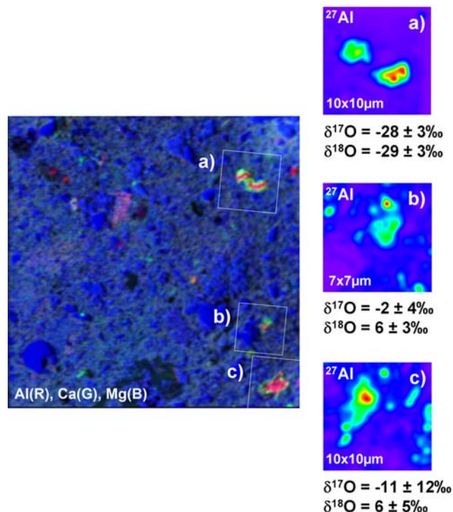
Fig. 6. NanoSIMS analysis to define the oxygen isotopic composition of three \mu\text{CAIs} in the area analyzed by ToF-SIMS. A ToF-SIMS map for Al, Ca, and Mg identifies the position of the \mu\text{CAIs} . In addition to analyzing for oxygen isotopes, ^{27}\text{Al} was imaged to confirm the locations of the CAIs in the NanoSIMS maps. In the NanoSIMS false color images on the right, the highest Al concentrations are shown in red.
