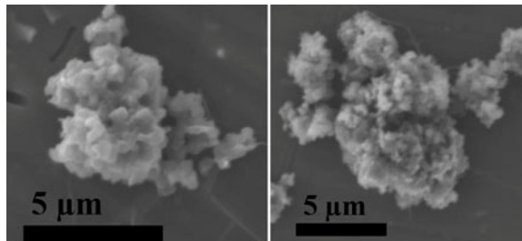
Fig. 1. Secondary electron images of fragments from the giant cluster IDP with surface morphology typical of CP-IDPs.
