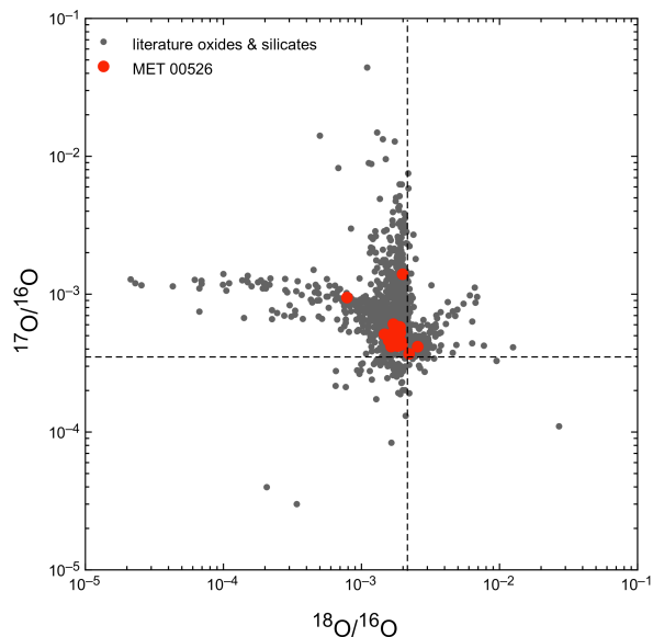
Figure 2. Oxygen three-isotope plot of presolar grains from MET 00526, compared with literature data.
