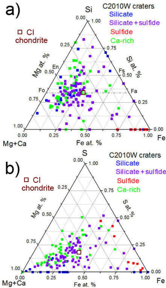
Fig. 2. Ternary composition diagram of Fe-Si-Mg (+Ca) and Fe-S-Mg (+Ca) showing the average composition of the surviving material in 130 C2010W Stardust craters along with CI chondrite average.
