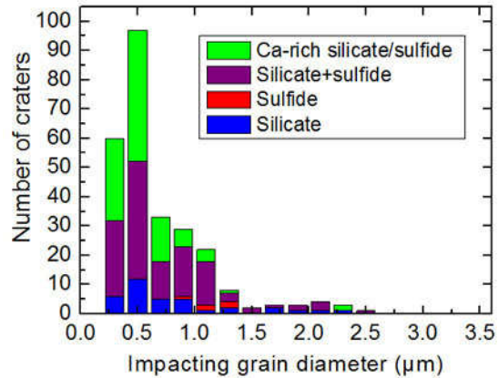
Fig.3 Impacting grain size distribution split by compositional type.
