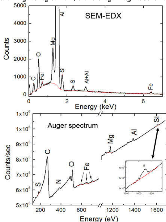
Fig.1. Representative SEM-EDX (a) and Auger electron (b) spectra (with inset Si peak) from a Stardust crater (C2010W f8-1c1), both of which show Mg, Si, Fe, and S peaks from cometary material. C, N and O peaks from unspattered Al foil surfaces are also seen.
