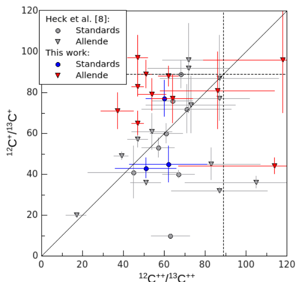
Fig. 3. Graphical summary of ^{12}\text{C}/^{13}\text{C} isotopic ratios determined by APT. Each data point represents the ratios of counts from an individual microtip. Errors are one \sigma , based on counting statistics. Dashed lines mark the terrestrial ^{12}\text{C}/^{13}\text{C} ratio of \sim 89 . The solid diagonal line indicates where equal ratios for singly- and doubly-charged C ions lie.
