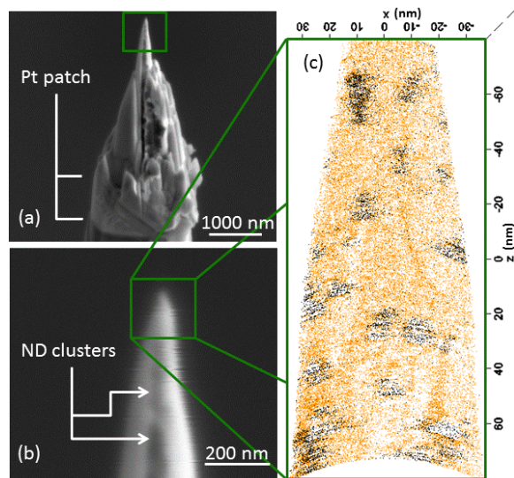
Fig. 1. (a) A microtip attached to a Si micropost by a Pt patch. (b) The same tip at higher magnification, displaying dark ND clusters in the deposition layer. (c) Cross-section of reconstructed APT data exhibiting individual NDs (black dots are C atoms) in a Pt matrix (orange dots).
