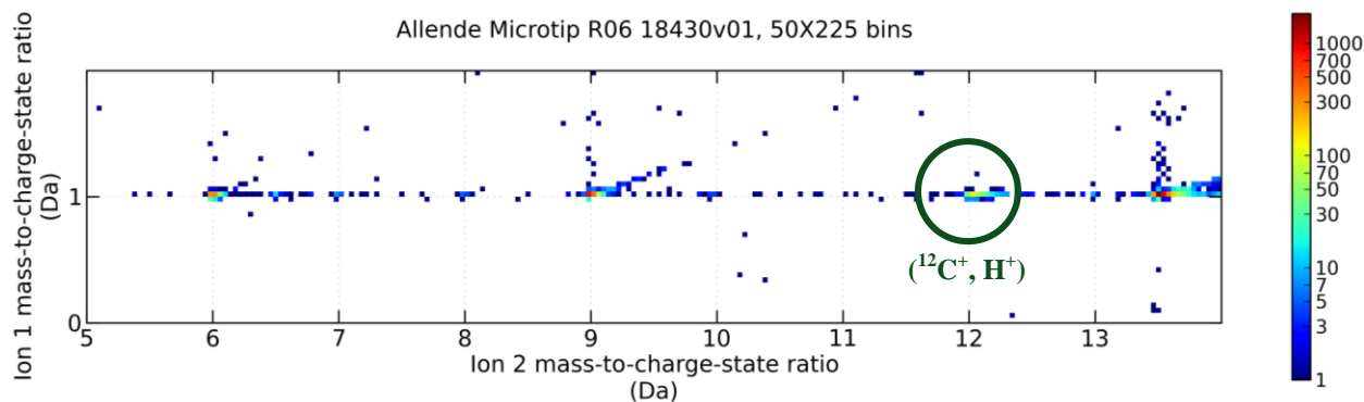
Fig. 2. 2D APT mass histogram plotting the mass-to-charge-state ratios of pairs of ions (double events) detected during the same laser pulse cycle. Hot spots correspond to ion species that tend to co-evaporate. Horizontal and vertical streaks represent a tendency for one ion in a pair to evaporate normally while the other evaporates shortly after the peak of the pulse. Diagonal lines represent pairs where both ions experience delayed evaporation. Visible in this range is the co-evaporation, or lack thereof, of H (1 Da) with C ions (6, 6.5, 12, 13 Da) and Al ions (9, 13.5 Da).
