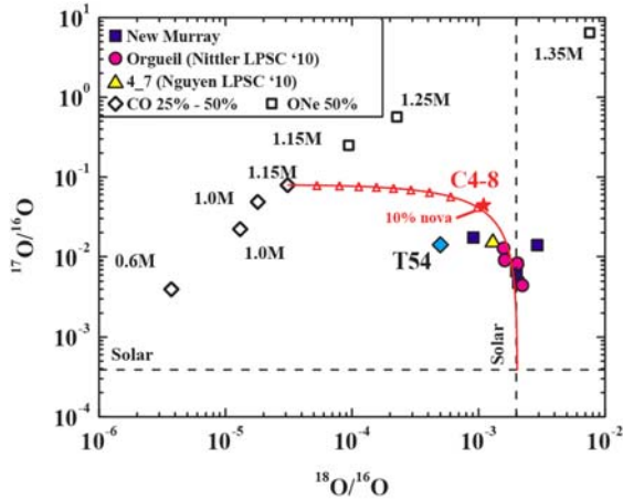
Figure 2. O-3 isotope plot of potential nova grains compared to new model predictions.
