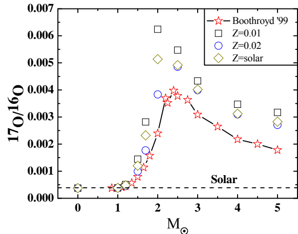
Figure 1. Theoretical ^{17}\text{O}/^{16}\text{O} ratios as a function of stellar mass calculated for several metallicities and compared to [12].
