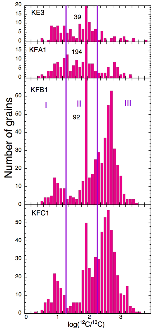
Fig. 1. Carbon isotopic distributions of Murchison graphite grains.
