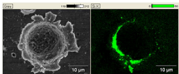
Fig.3. Image and extracted Si x-ray map from a Si-rich crater. Uneven distribution of Si counts on left side is an EDXS count rate artifact (crater wall facing detector has enhanced counts).
