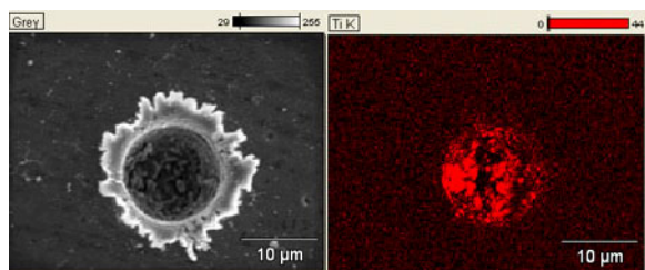
Fig. 2. Image and extracted Ti x-ray map from a typical Ti-rich crater.
