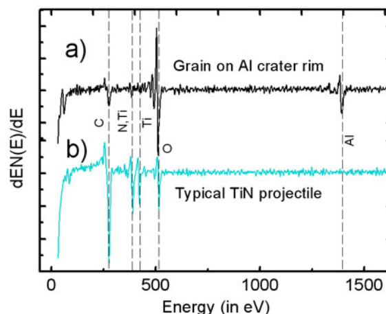
Fig 4. Derivative Auger energy spectra of a) grain on Al crater rim showing N and Ti peaks and b) typical raw TiN projectile showing considerably stronger N and Ti. The strong C peak from the TiN projectile is presumably due to thin surface contamination.
