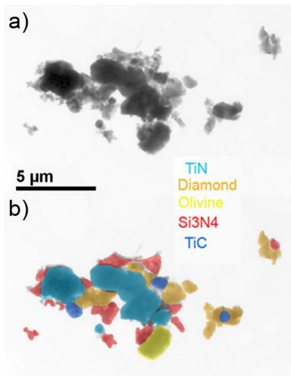
Fig.1. a) Bright-field image of typical fragment from the refractory grain mix projectile material and b) same fragment with phases identified with color code.
