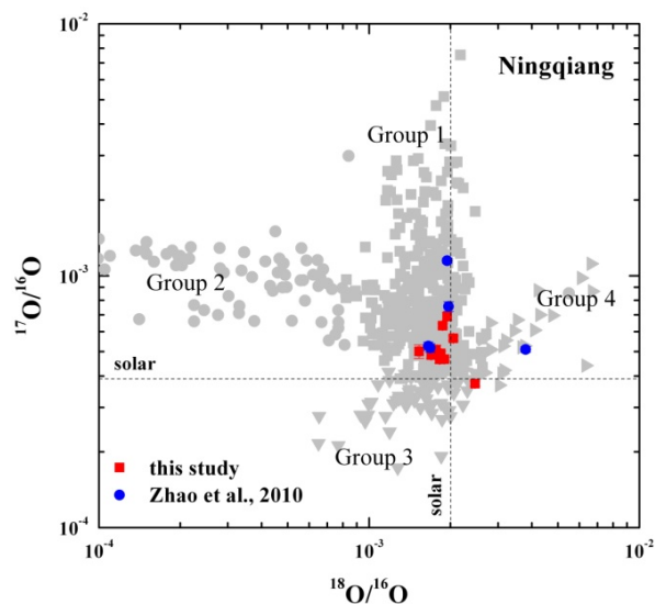
Figure 1. Oxygen three-isotope plot showing O-anomalous grains from Ningqiang. Error bars are 1\sigma . Other data (gray dots) are from the Presolar Grain Database [9].
