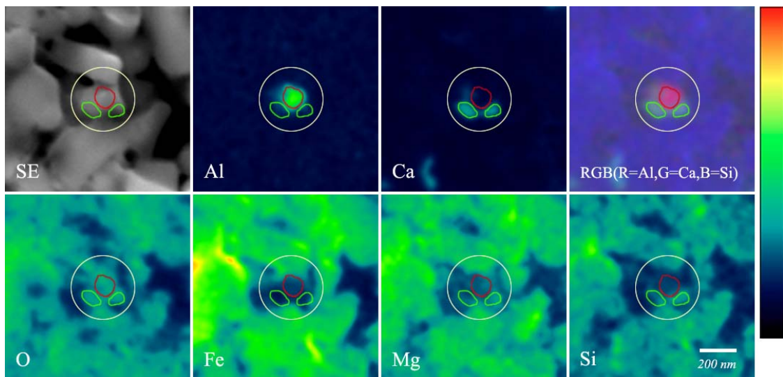
Fig 2. Secondary electrons and Auger elemental maps of the complex grain (white circle) from Ningqiang. (Al-rich oxide, red circle; Ca-rich silicates, green circle)
