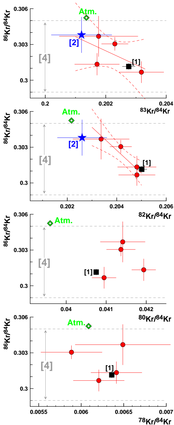
Fig.2. Red circles are Kr from total UV-laser extraction (this work). These data are not corrected for blank contribution and for doubly charges ^{40}\text{Ar} . Black squares [1] are most accurate regolith data by Pepin, Becker and Rider, 1995. Blue stars [2] are data by Pederoni and Begemann, 1994. Grey [4] is the only published ^{86}\text{Kr}/^{84}\text{Kr} ratio recently measured in Genesis collectors by Heber et al, 2006. All error bars are 2\sigma . Confidence intervals for correlation lines are 90%.
