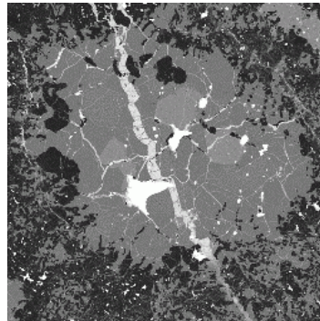
Figure 2: Equigranular ol-opx-cpx rock surrounded by graphite-rich lithologies. Bright phase is metal, vein is filled with rust. BSE picture; width ~3 mm.
