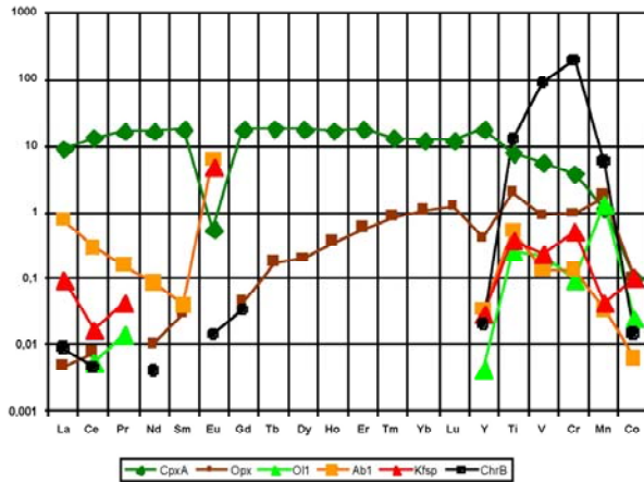
Figure 6: CI-normalized [7] trace element abundances in major phases of CC inclusion SiGrMet05.
