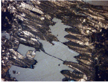
Figure 5: Detail of thin vein consisting of metal (gray) intergrown with feathery graphite growing from the crack wall. Optical picture, partly crossed polarizers, width ~680 μm.
