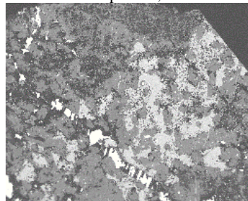
Figure 3: Chromite-rich lithology (light gray) with graphite-rich ones (upper center-left and lower right corner) cut by metal-graphite vein (from upper left to lower right). BSE picture; width ~11.5 mm.
