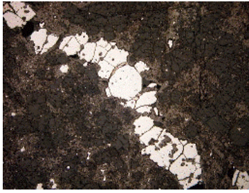
Figure 4: Granular metal vein (white) contains cliftonite and schreibersite and cuts through silicate-graphite rocks. Reflected light optical photograph, width ~7 mm.
