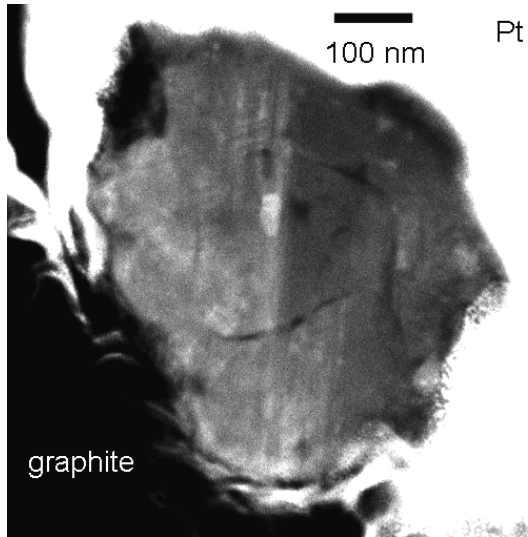
Figure 1. Z-contrast image of SiC grain 23. High atomic number areas appear bright and low atomic number areas appear dark in this image mode. The grain shows significant internal composition variation, as indicated by the bright and dark subgrains, planar striations, and a dark triangular boundary. The oxide rim is a dark band 10 to 30 nm thick around the exterior of the grain.
